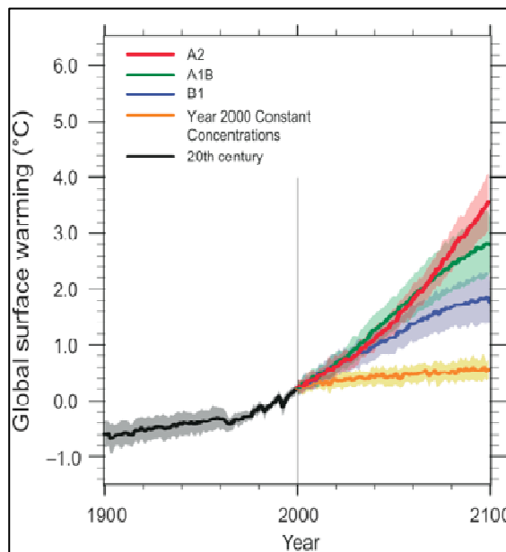
Figure 4.3. Projected future global temperature change for the SRES emission scenarios (degrees Celsius). The range for each individual emission scenario indicates model uncertainty in simulating the response of the Earth system to human emissions of greenhouse gases (IPCC 2007b.).
