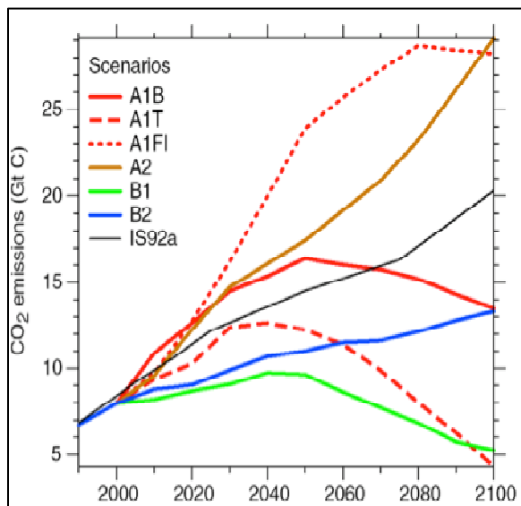
Figure 4.1. Projected future carbon emissions for the SRES emission scenarios. Emissions for the higher scenario (A1FI) corresponds to the red dotted line, while emissions for the lower (B1) scenario are indicated by the solid green line (Nakicenovic et al. 2000).
