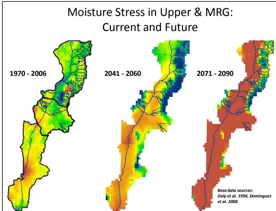
Figure C3.1. 1970-2006 = trend in moisture deficit for the Upper and Middle Rio Grande (MRG); Preliminary future forecasts: 2041-2060=departure (difference) in deficit relative to 1951-2006 baseline; 2071-2090=departure in deficit relative to 51-06 baseline (Bosque Working Group 2009).
