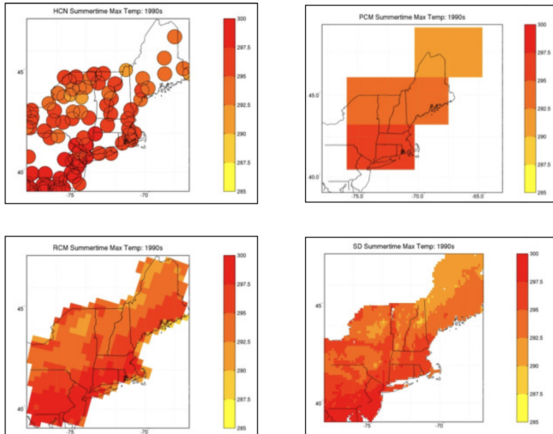
Figure 4.4. Average summer maximum temperature in the US Northeast for the 1990s, based on (a) observations from weather stations in the Historical Climatology Network, (b) the global climate model PCM, (c) regional climate model simulations, and (d) statistically downscaled simulations. From Hayhoe et al. (2008).
