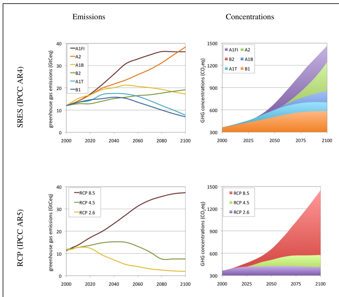
Figure 4.2. Projected future CO 2 -equivalent emissions and concentrations for the SRES emission scenarios (IPCC AR4) and Representative Concentration Pathways (IPCC AR5).
