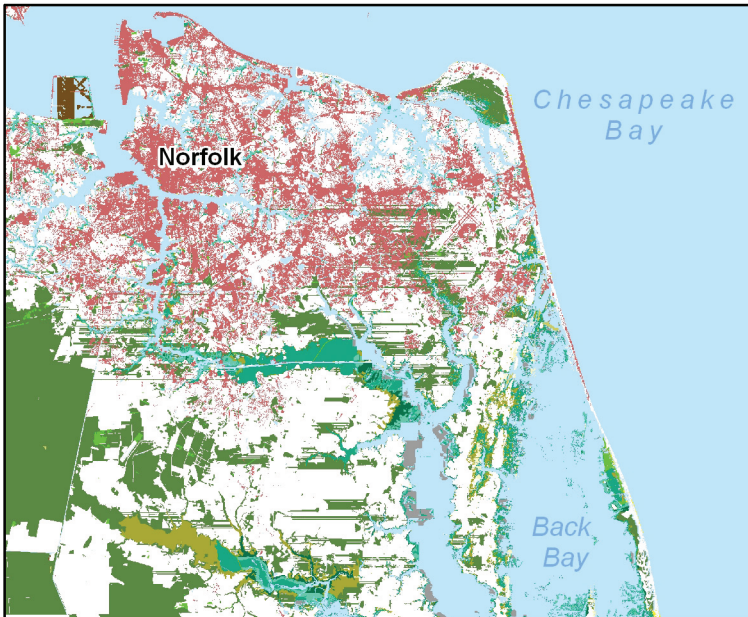
Year 2100 (27.2 inches)
