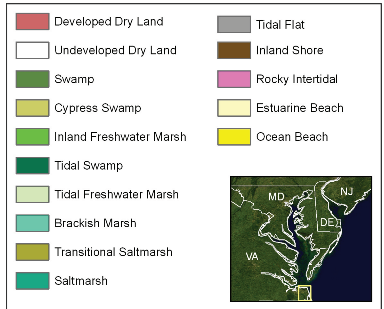
Year 2050 (11.2 inches)
