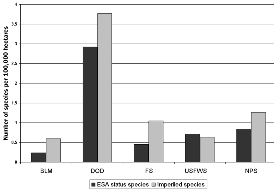
Figure 3. Density of endangered and imperiled species on federal agency lands. Calculating the density of species per 100,000 hectares highlights the disproportionate role that DOD lands play in sustaining the nation's biodiversity. Military lands have three times higher densities of ESA status and imperiled species than do lands of the NPS, the second-ranked agency for densities of both ESA and imperiled species. Source: NatureServe Central Databases (based on data from US natural heritage programs), February 2007. Abbreviations: BLM, Bureau of Land Management; DOD, Department of Defense; FS, Forest Service; NPS, National Park Service; USFWS, US Fish and Wildlife Service.
