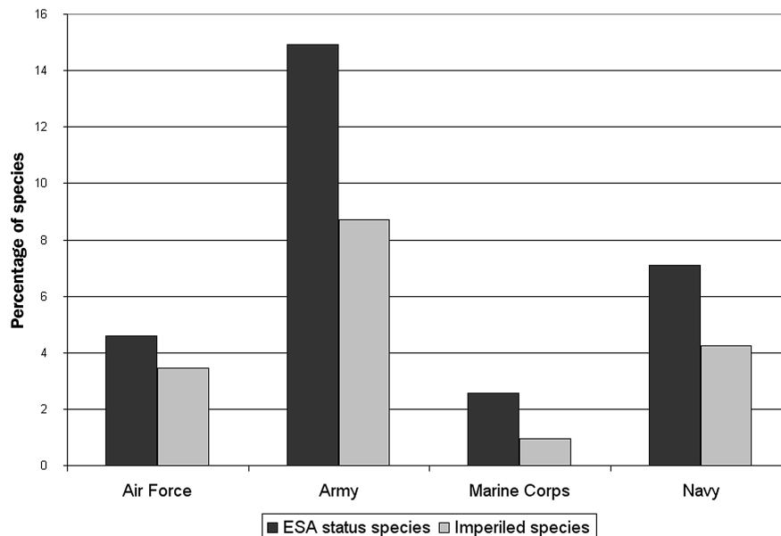
Figure 4. Distribution of endangered and imperiled species by military service. Army lands harbor more than twice the number of ESA status and imperiled species as those of the navy, which supports the next highest number. Source: NatureServe Central Databases (based on data from US natural heritage programs), February 2007.
