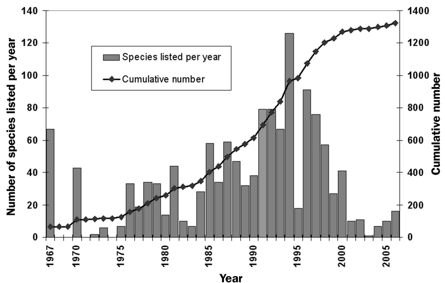
Figure 1. Listings under the US Endangered Species Act. The pace of listings under the ESA has varied considerably over time, primarily reflecting availability of funding for listing activities and shifts in policy. As of October 2007 a total of 1333 US species and populations were listed as threatened or endangered under the act. Under the ESA, listings can apply to species, infraspecific taxa, or, for vertebrate animals, "distinct population segments." Source: US Fish and Wildlife Service, Threatened and Endangered Species System, October 2007.
