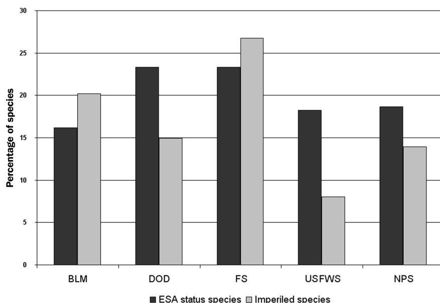
Figure 2. Distribution of endangered and imperiled species on federal agency lands. Lands of the DOD and USDA Forest Service harbor the greatest number of species with status under the Endangered Species Act (23%), while Forest Service lands support the largest number of NatureServe-assessed imperiled species (27%). Source: NatureServe Central Databases (based on data from US natural heritage programs), February 2007. Abbreviations: BLM, Bureau of Land Management; DOD, Department of Defense; FS, Forest Service; NPS, National Park Service; USFWS, US Fish and Wildlife Service.
