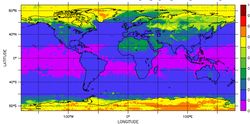
Monthly TOA Clear-sky Albedo (CERES EBAF) (fraction)
