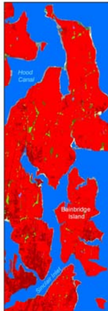
Year 2100, A1B-Max
