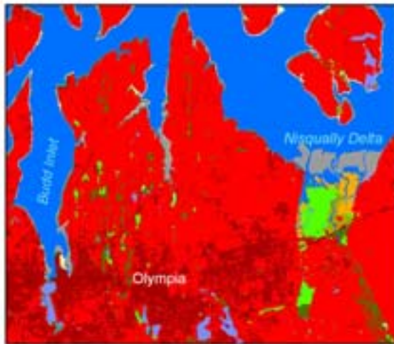
Year 2050, A1B-Max
